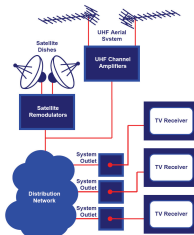
Figure 2: Block diagram of a SMATV system
