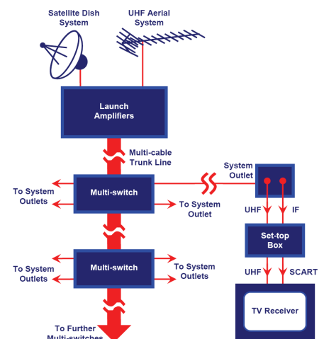
Figure 3: Block diagram of an Integrated Reception System (IRS)
