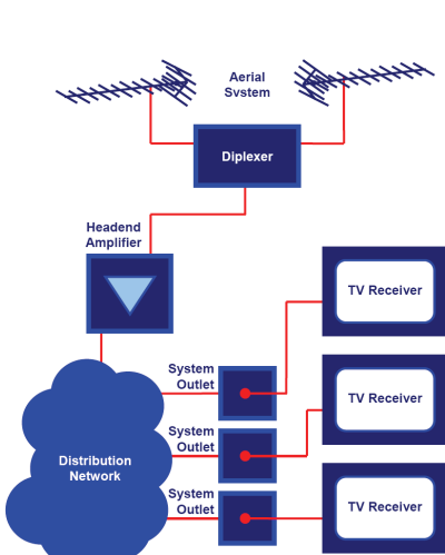
Figure 1: Block diagram of an MATV system
